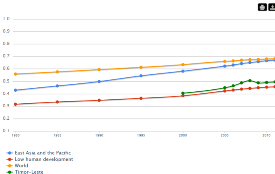
Human Development Index: Trends 2000 - present
